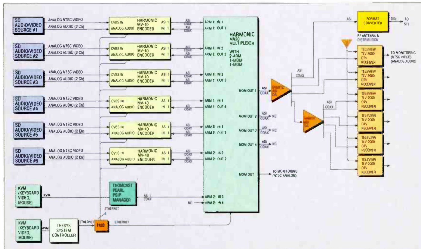
Paxson's WCPX-DT is multicasting six channels of programming in its allotted 6MHz. The station employs Harmonic encoding and multiplexing equipment, Evertz DAs and Thomcast's Pearl PSIP manager.
