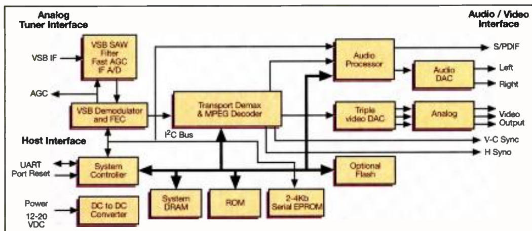
M-DTV module includes an ATSC receiver, a legacy converter, digital audio and a system processor to oversee the system.
