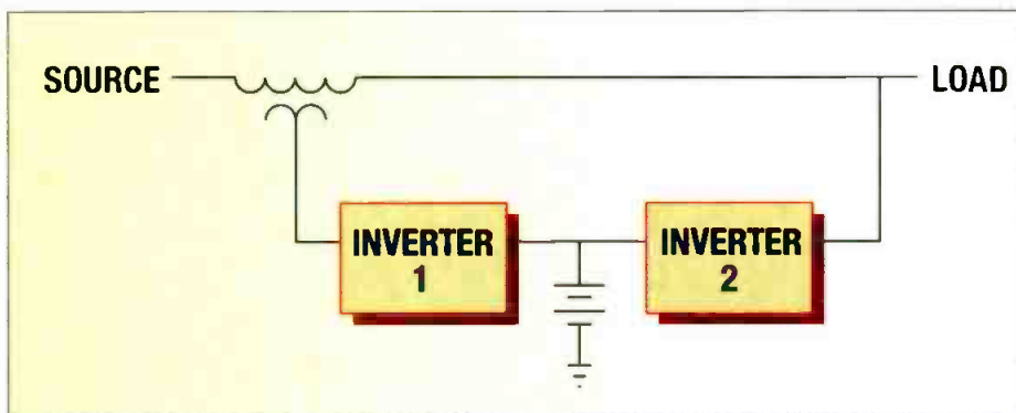
Figure 4. In a delta conversion configuration, a second two-way inverter can either add voltage to the transformer tap or act as an additional load to lower the current out.
