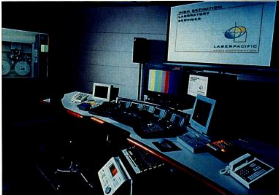
Telecine suites are a crucial link in creating a 24 p master, syncing timecode, audio and generating a database for offline editing systems. LaserPacific's Telecine 1 (one of four Philips Spirit bays) was built as a multiformat mastering room.
