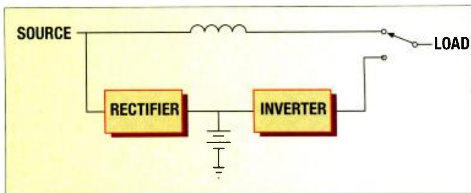
Figure 1. Lower-end UPS systems are likely to employ an offline UPS configuration, which simply opens the path from the battery in the event of a power failure.
