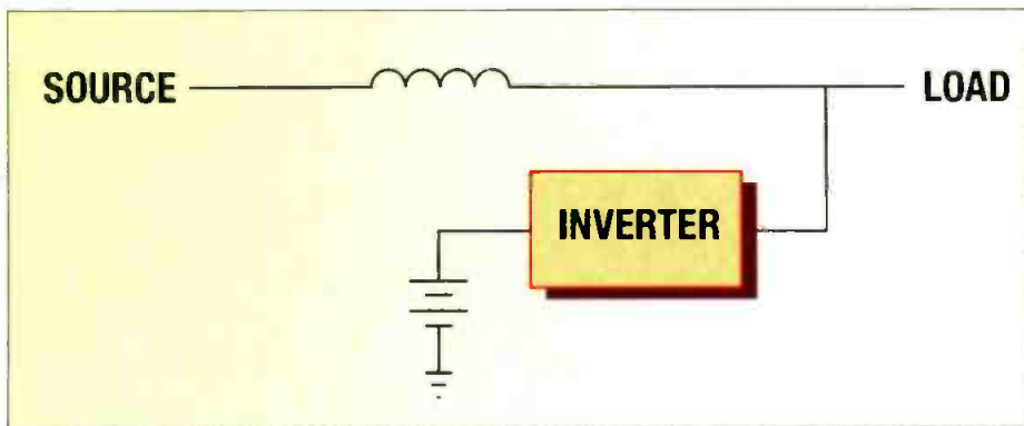
Figure 3. In a single conversion UPS, separate rectifiers and inverters are replaced by an inverter/rectifier that passes power both to the battery and back out again to load.
