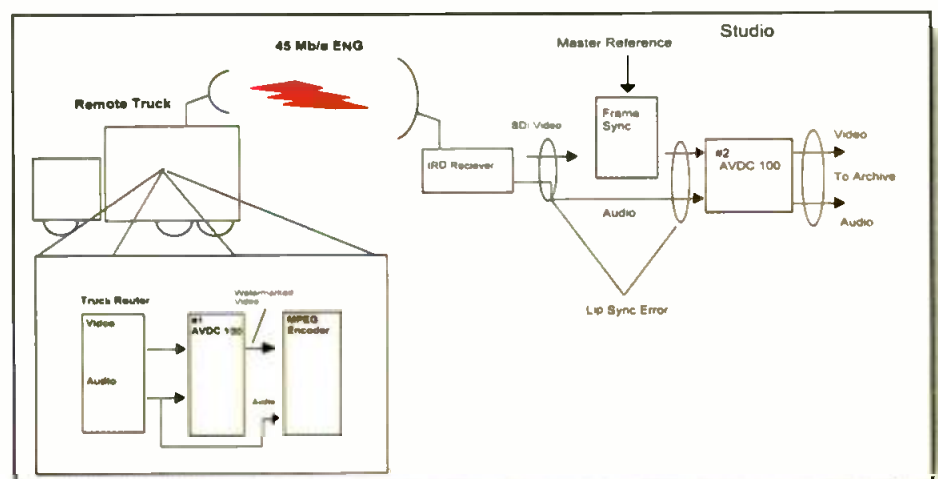
Figure 1. Two AVDC100s utilized together to monitor and correct lip-sync in remote production. One system operates in encoder mode in a remote production truck, and the other is installed in the studio in decode and lip-sync correct mode.
