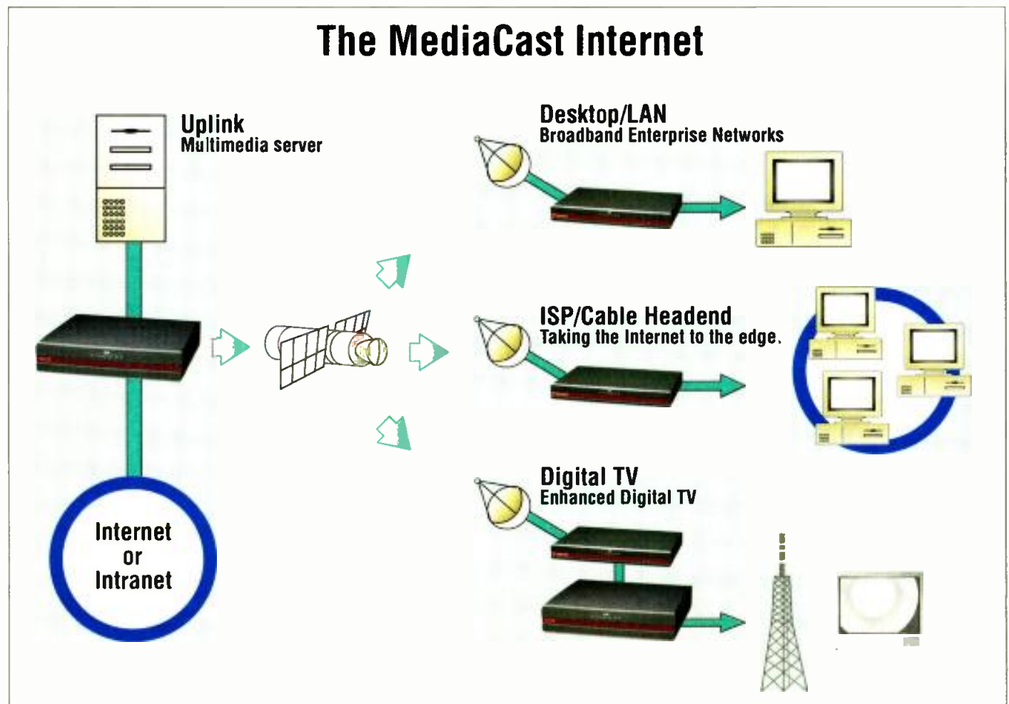
Figure 1. In multicasting applications, data is transferred from the Forte gateway to the IP-COMPANION via satellite and output as IP data via an Ethernet 10/100BaseT interface to a desktop, LAN or Internet headend.
