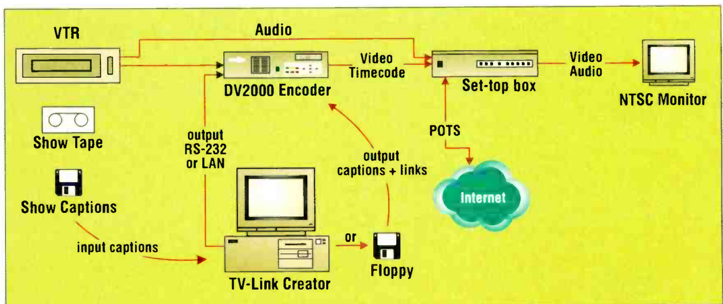
Figure 2. Authoring interactive content includes a two-step process that takes previously encoded captions and adds interactive content through an encoding system and software.
