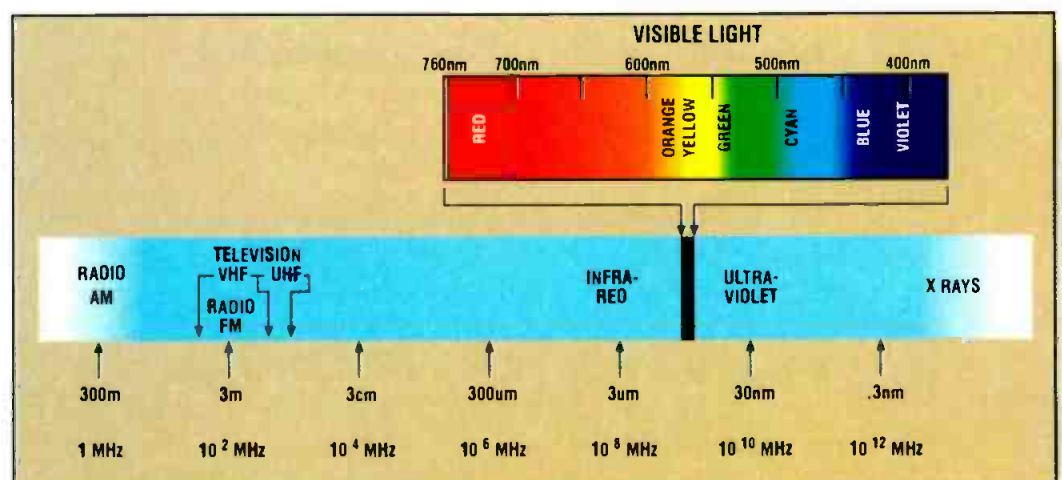
Figure 3. The spectrum of electromagnetic radiation includes the AM & FM radio bands, VHF and UHF television frequencies as well as visible light.
