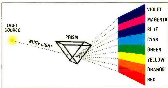
Figure 1. When passed through a prism, white light can be split into spectral colors.
