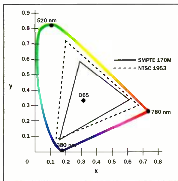
Figure 4. The CIE color diagram is representative of all visible colors. The chart above includes the primary red, blue and green colors used for SMPTE 170M and those chosen in 1953 for NTSC.
