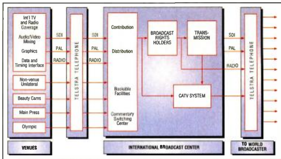
Content flows from the various venues to the IBC, then from the IBC to the individual rights holders via Telstra fiber and codecs.
